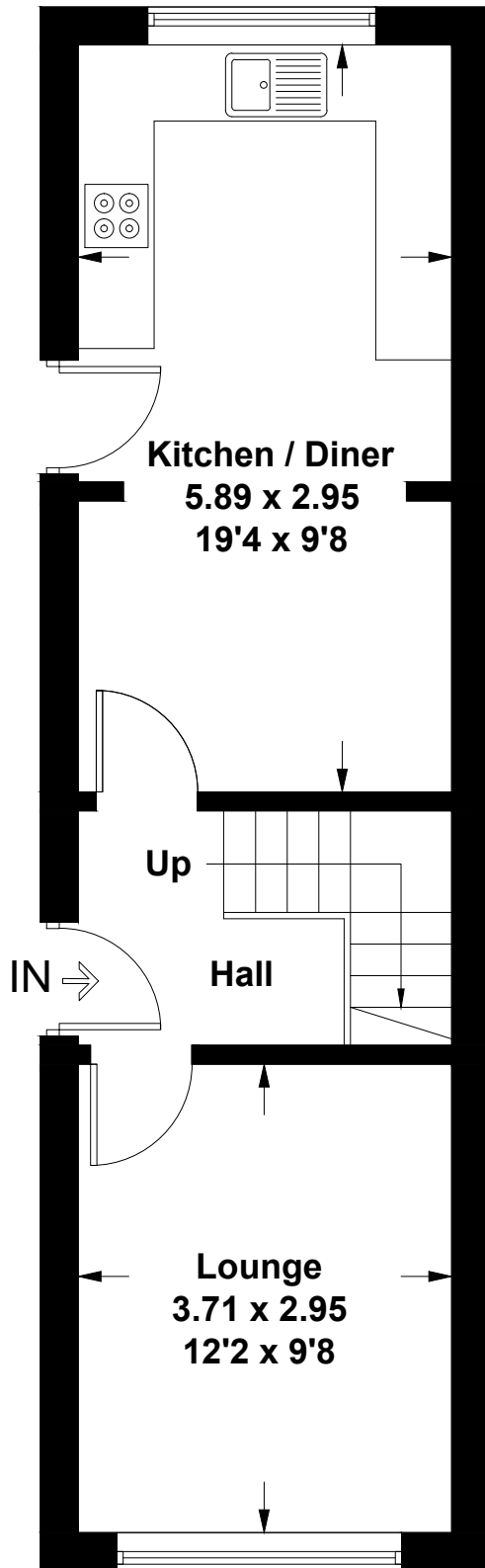
Ground Floor
